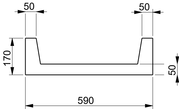
Section VIEW C077
