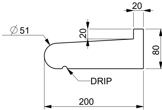
SECTION VIEW W007
