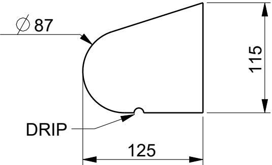
SECTION VIEW W001
