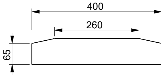
Section VIEW C069
