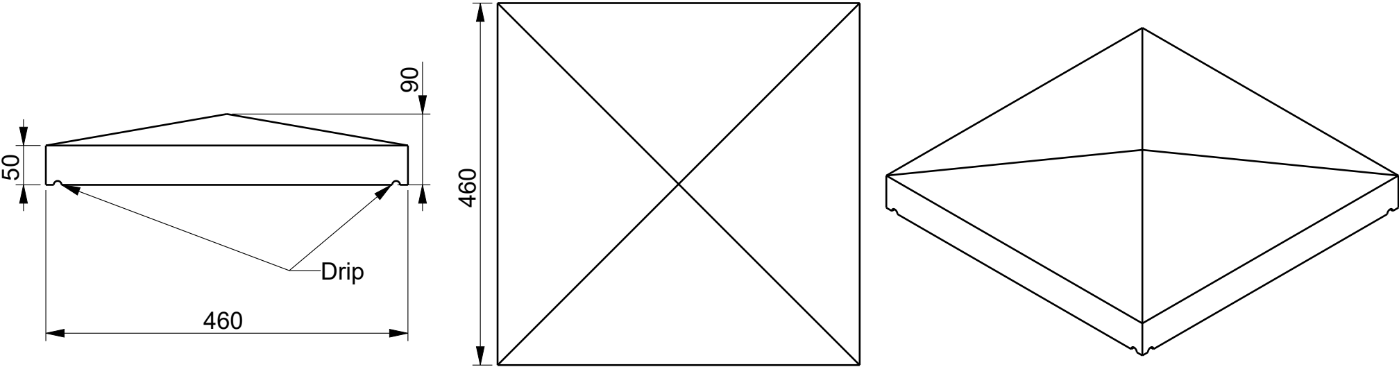
SECTION VIEW
